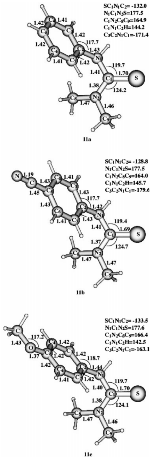
Figure 2. Optimized geometries of thioureas 11a–c ; lengths in Å, angles in ^\circ .
