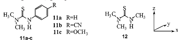
Scheme 4. The thioureas under study
