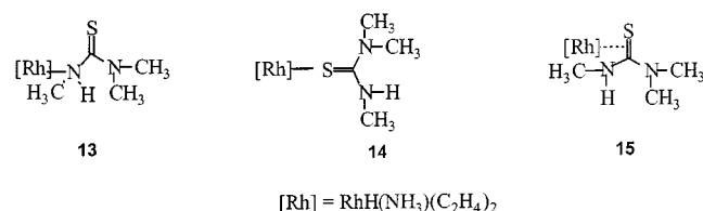
Scheme 5. Various coordination modes of thiourea 12 towards rhodium
