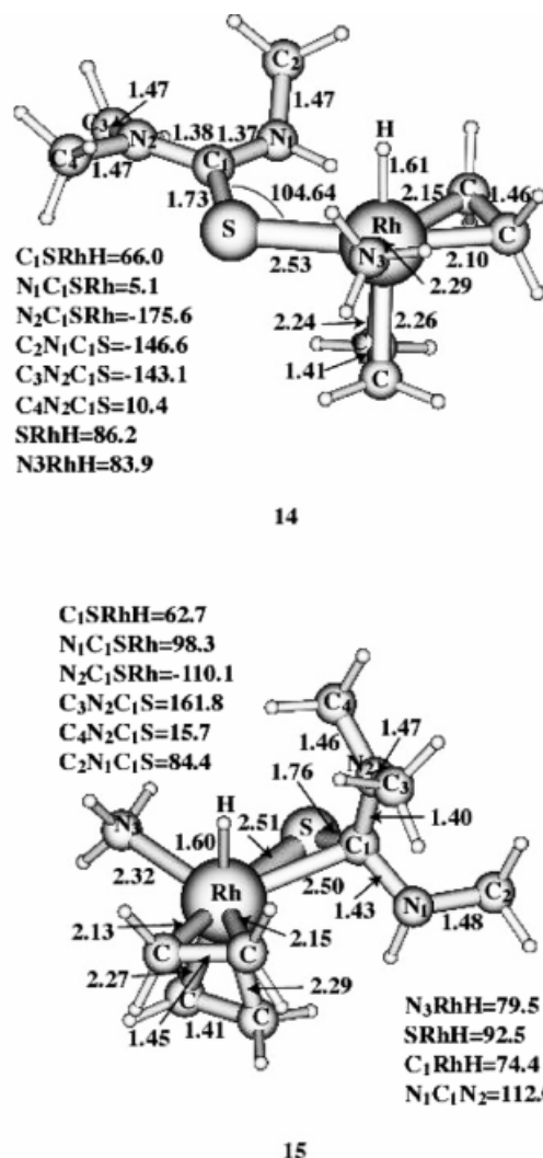
Figure 1. Optimized geometries of rhodium complexes 14 and 15 ; lengths in Å, angles in °
