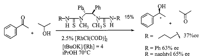
Scheme 1. Enantioselective hydride-transfer reduction of acetophenone using dithiurea ligands
